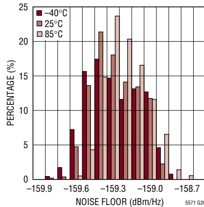
Noise Floor Distribution (no RF)
