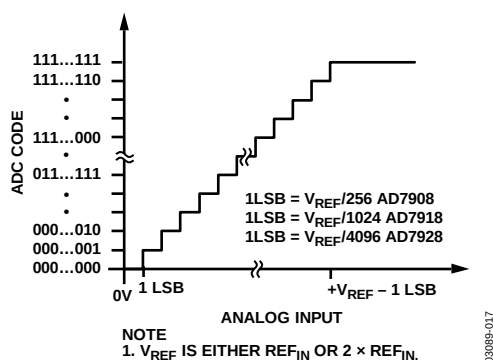
Figure 17. Straight Binary Transfer Characteristic
