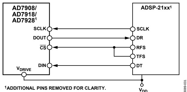
Figure 31. Interfacing to the ADSP-21xx
