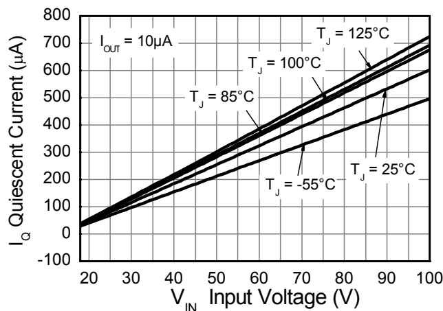
Quiescent Current
