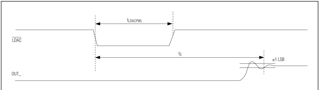
Figure 14. LDAC Functionality
