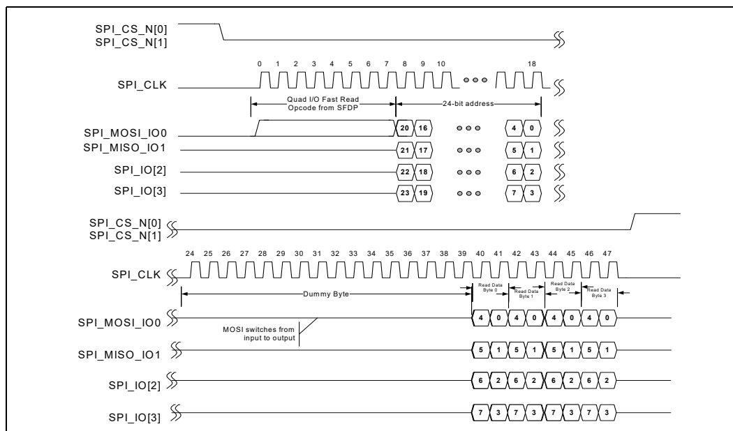
Figure 19-9. Quad-I/O-Fast-Read Timing
