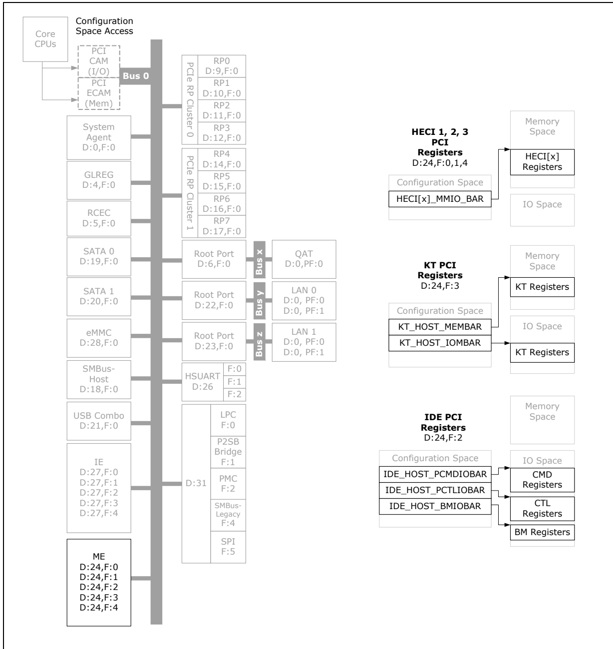
Figure 36-2. Register Map
