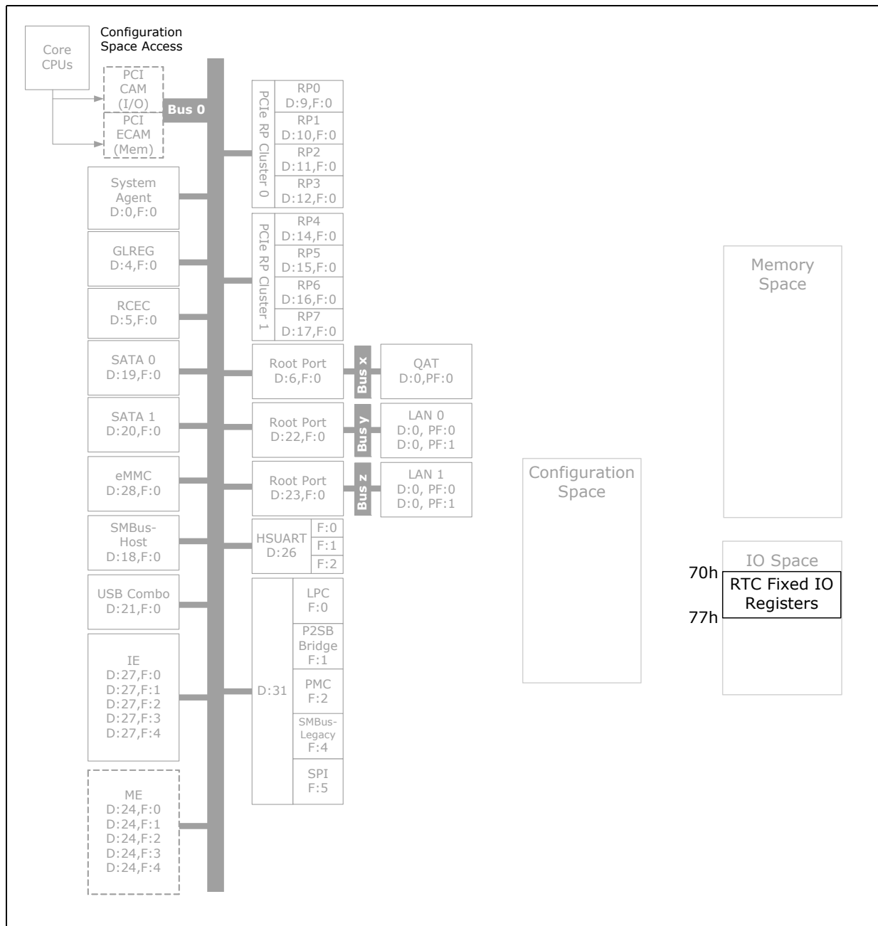
Figure 24-2. Register Map
