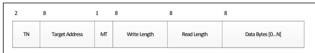
Figure 30-5. PECI Message Header in the SMBus Packet
