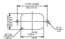
SUGGESTED MOUNTING CUTOUT (MOUNTING FROM BEHIND)
