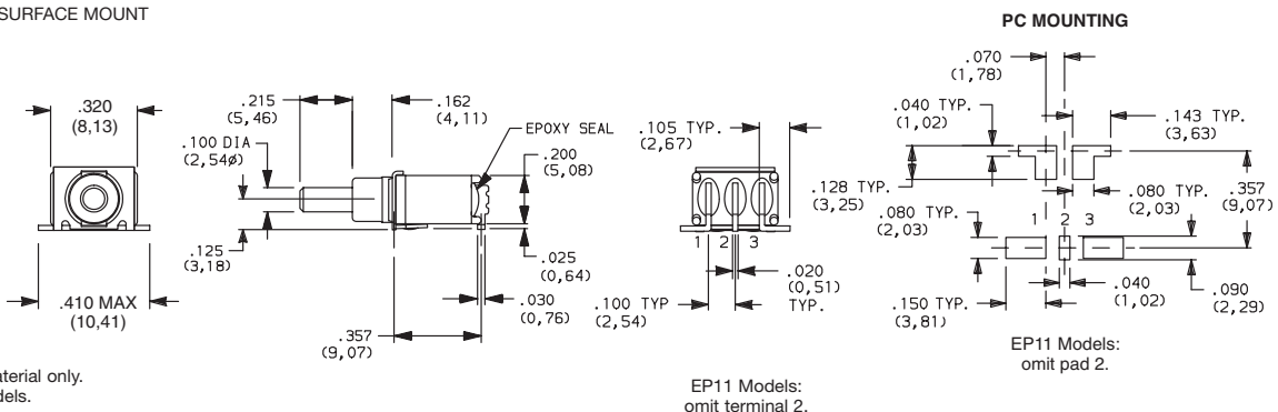
EP12SD1SAPE SPDT
