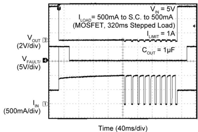
Output Thermal Shutdown &amp; Recovery
