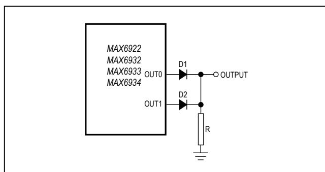
Figure 5. Paralleling Outputs
