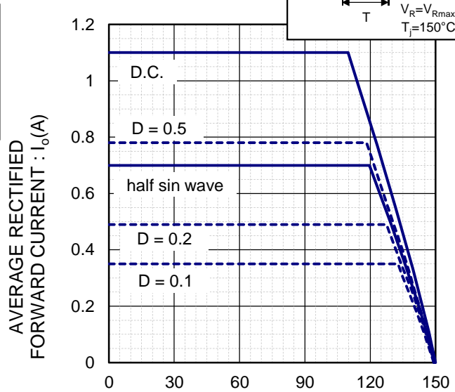
LEAD TEMPERATURE : T_l ( ^{\circ} C) DERATING CURVE ( I_o - T_l )
