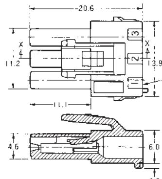
Section X-X
