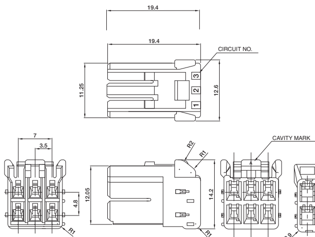
Plug Housing (For Receptacles)
