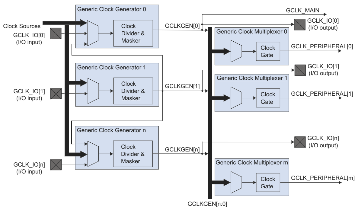
Figure 14-2. Generic Clock Controller Block Diagram (1)
