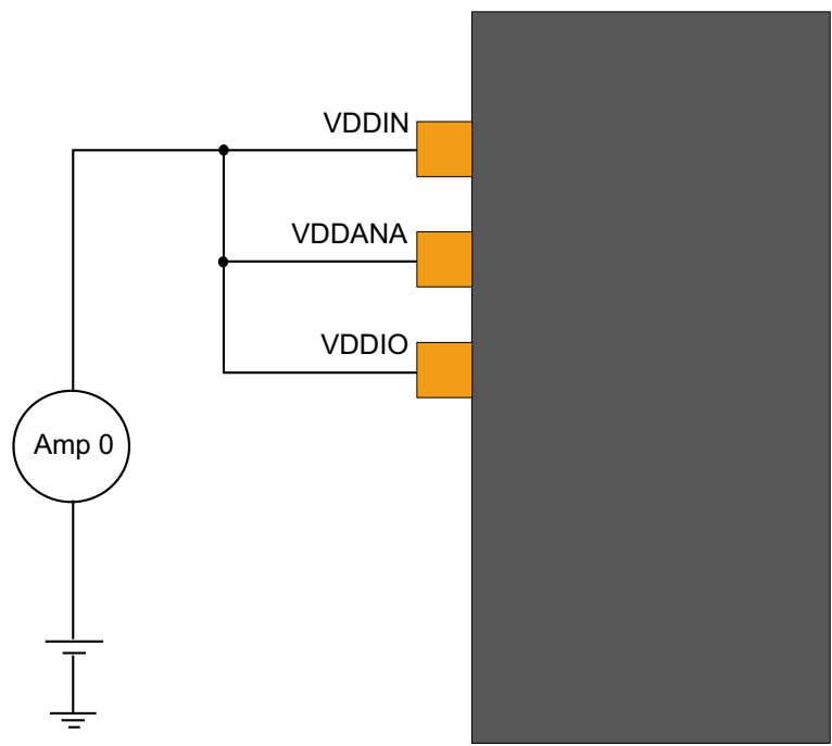
Figure 39-1. Measurement Schematic
