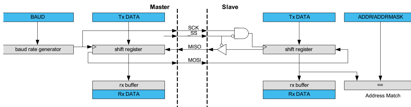
Figure 26-1. Full-Duplex SPI Master Slave Interconnection
