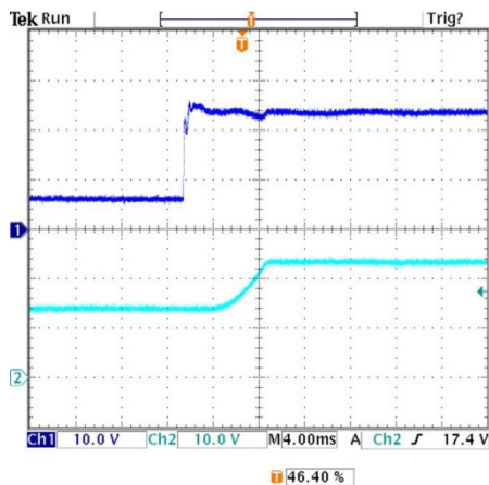
Pre-biased output voltage added connecting an external 680\mu F to the output ( V_{in}=24V , I_{out}=0A , +25^\circ C )
