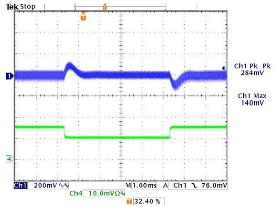
Step Load Transient Response ( V_{in}=24V , V_{out}=nom. , I_{out}=50-75-50\% of full load, C_{load}=2000\mu F , T_a=+25^\circ C. , ScopeBW=20MHz)
