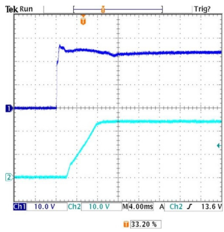
Power On Startup Delay ( V_{in}=0 to 24V , V_{out}=nom. , I_{out}=2A , C_{load}=0\mu F , T_a=+25^\circ C. , ScopeBW=20MHz) Trace 1= V_{in} , Trace 2= V_{out}
