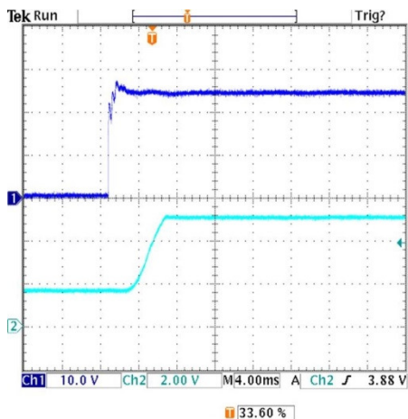
Pre-biased output voltage added connecting an external 5000µF to the output ( V_{in}=24V , I_{out}=0A , +25^\circ C )
