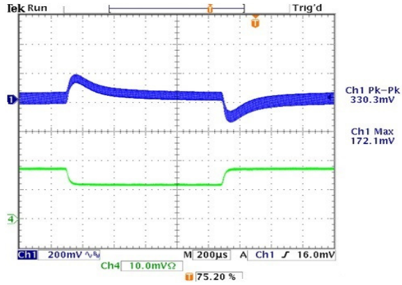
Step Load Transient Response ( V_{in}=24V , V_{out}=nom. , I_{out}=50-75-50\% of full load, C_{load}=1\mu F ceramic || 10\mu F tantalum, T_a=+25^\circ C. , ScopeBW=20MHz)
