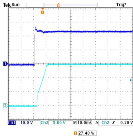
Power On Startup Delay ( V_{in}=0 to 24V, V_{out}=\text{nom.} , I_{out}=3.3A , C_{load}=0\mu\text{F} , T_a=+25^\circ\text{C} ., ScopeBW=20MHz) Trace 1= V_{in} , Trace 2= V_{out}
