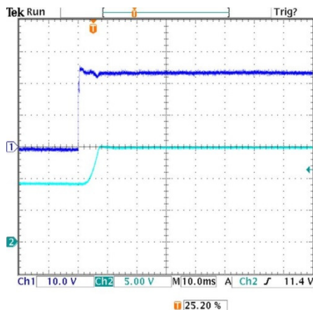
Pre-biased output voltage added connecting an external 2000uF to the output ( V_{in}=24V , I_{out}=0A , +25^\circ\text{C} )
