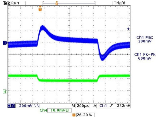
Step Load Transient Response ( V_{in}=24V , V_{out}=\text{nom.} , I_{out}=50\text{-}75\text{-}50\% of full load, C_{load}=1\mu\text{F} ceramic II 10\mu\text{F} tantalum, T_a=+25^\circ\text{C} ., ScopeBW=20MHz)
