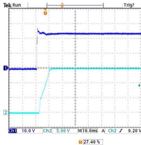
Power On Startup Delay ( V_{in}=0 to 24V , V_{out}=\text{nom.} , I_{out}=3.3A , C_{load}=0\mu\text{F} , T_a=+25^\circ\text{C} ., ScopeBW=20MHz) Trace 1= V_{in} , Trace 2= V_{out}
