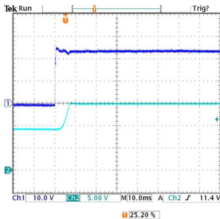
Pre-biased output voltage added connecting an external 2000uF to the output ( V_{in}=24V , I_{out}=0A , +25^\circ C )
