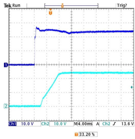
Power On Startup Delay ( V_{in}=0 to 24V , V_{out}=\text{nom.} , I_{out}=2A , C_{load}=0\mu\text{F} , T_a=+25^\circ\text{C.} , ScopeBW=20MHz) Trace 1= V_{in} , Trace 2= V_{out}
