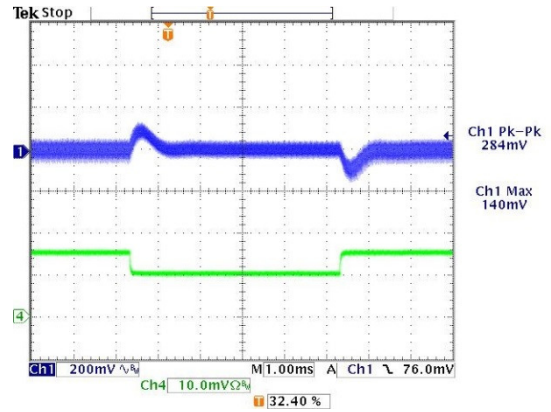
Step Load Transient Response ( V_{in}=24V , V_{out}=\text{nom.} , I_{out}=50\text{-}75\text{-}50\% of full load, C_{load}=2000\mu\text{F} , T_a=+25^\circ\text{C.} , ScopeBW=20MHz)
