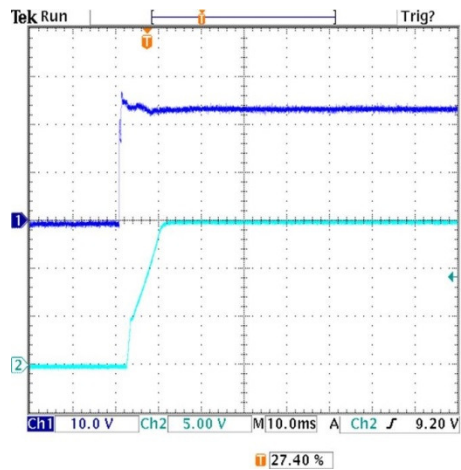
Power On Startup Delay ( V_{in}=0 to 24V, V_{out}=nom. , I_{out}=3.3A , C_{load}=0\mu F , T_a=+25^\circ C. , ScopeBW=20MHz) Trace 1= V_{in} , Trace 2= V_{out}
