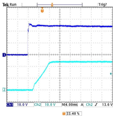
Power On Startup Delay ( V_{in}=0 to 24V , V_{out}=\text{nom.} , I_{out}=\text{no load} , C_{load}=0\mu\text{F} , T_a=+25^\circ\text{C.} , ScopeBW=20MHz) Trace 1= V_{in} , Trace 2= V_{out}
