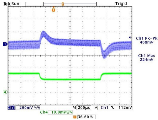
Step Load Transient Response ( V_{in}=24V , V_{out}=\text{nom.} , I_{out}=50\text{-}75\text{-}50\% of full load, C_{load}=1\mu\text{F} ceramic II 10\mu\text{F} tantalum, T_a=+25^\circ\text{C.} , ScopeBW=20MHz)
