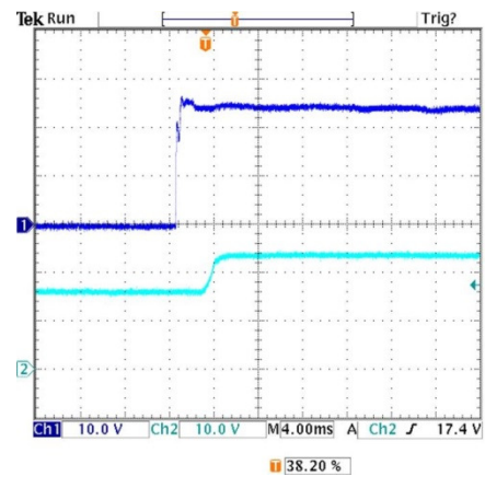
Pre-biased output voltage added connecting an external supply through a diode ( V_{in}=24V , I_{out}=0A , +25^\circ\text{C} )
