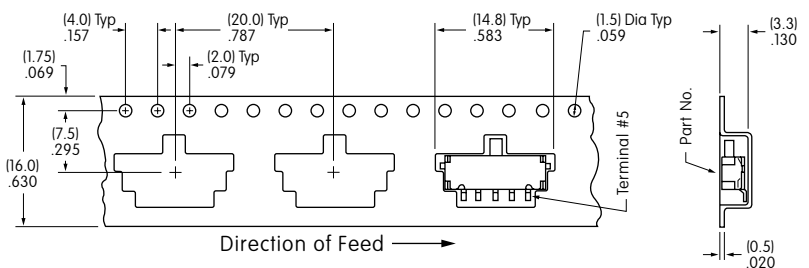
Tape Dimensions
