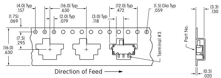
Tape Dimensions
