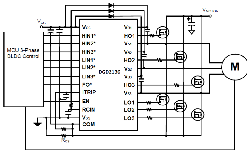
Typical Configuration
