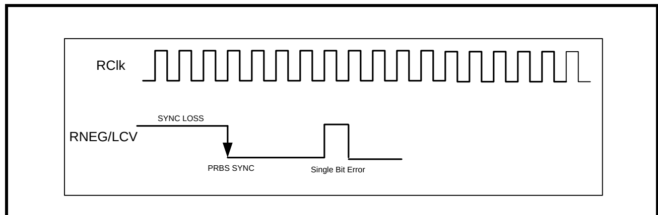
FIGURE 25. PRBS MODE
