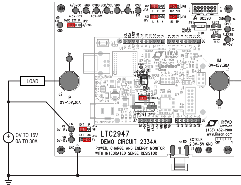
Figure 2. Linduino Shield Style Hardware Bench Setup
