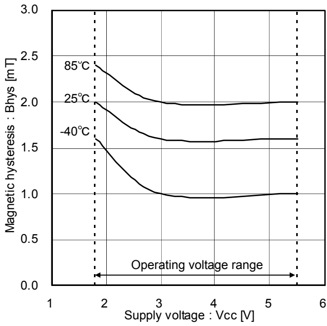
Figure 7. Magnetic hysteresis
