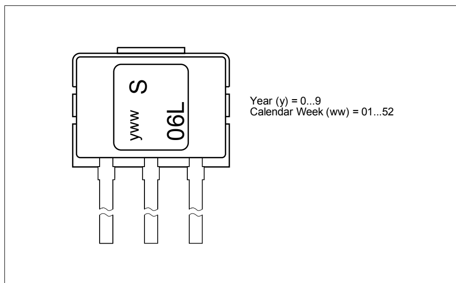
Figure 5 Marking TLE4906L
