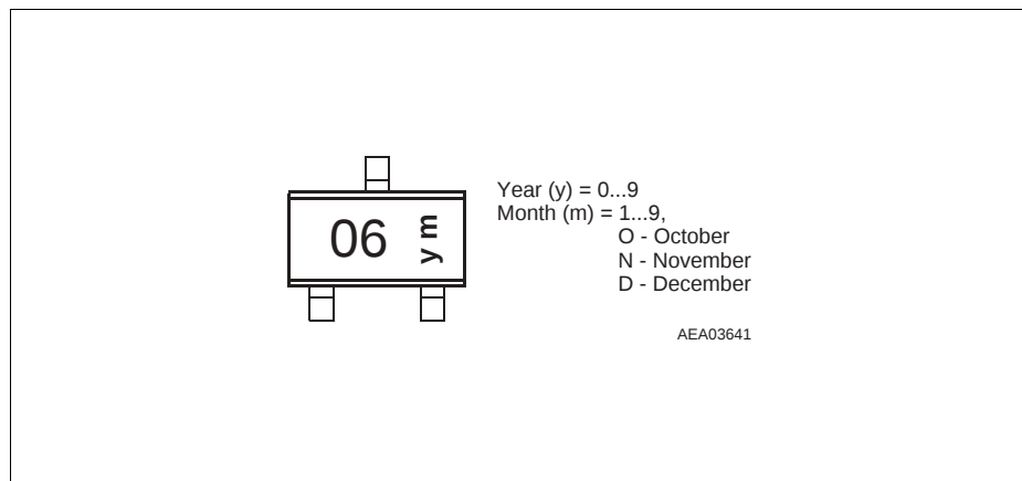
Figure 4 Marking TLE4906H
