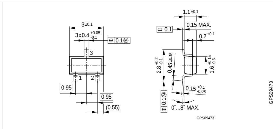
Figure 8 SC59
