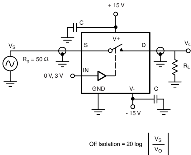
Figure 4. Off Isolation
