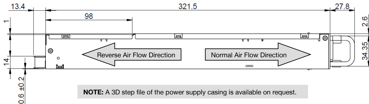
Figure 43 - Side View 1
