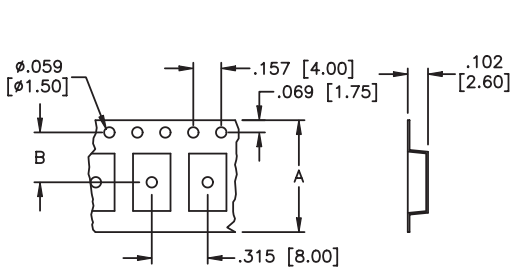
CARRIER TAPE
