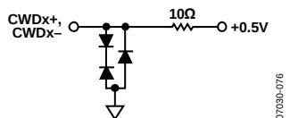
Figure 36. Equivalent CWDx± Output Circuit
