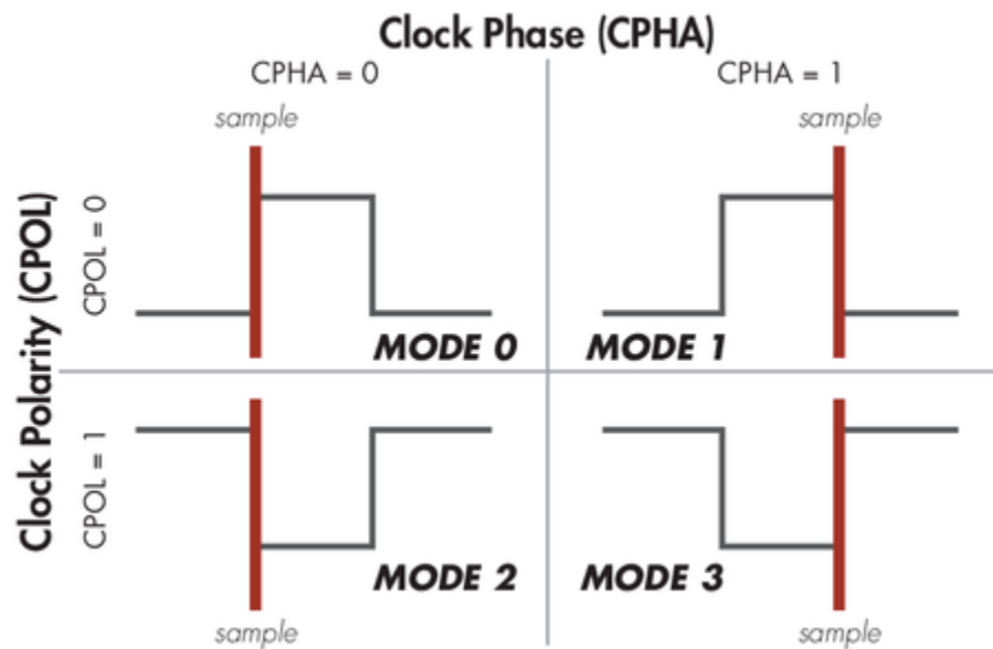
Figure 26 : SPI Modes
