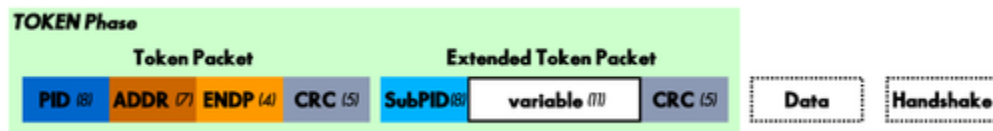
Figure 17 (above) : Extended Token Transaction
