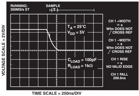
TPC 3. TMP03 Output Fall Time at 25^\circ C
