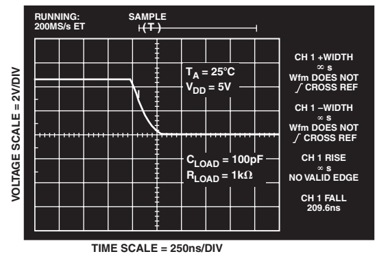
TPC 3. TMP03 Output Fall Time at 25^\circ C
