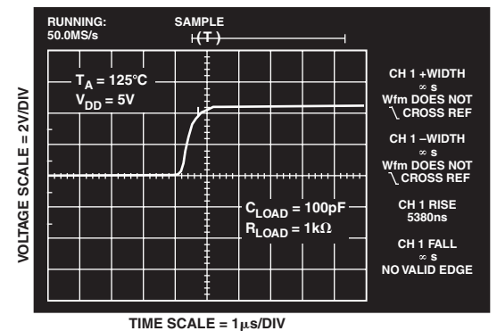
TPC 6. TMP03 Output Rise Time at 125^\circ C
