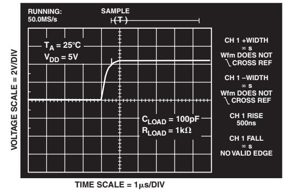
TPC 5. TMP03 Output Rise Time at 25^\circ C
