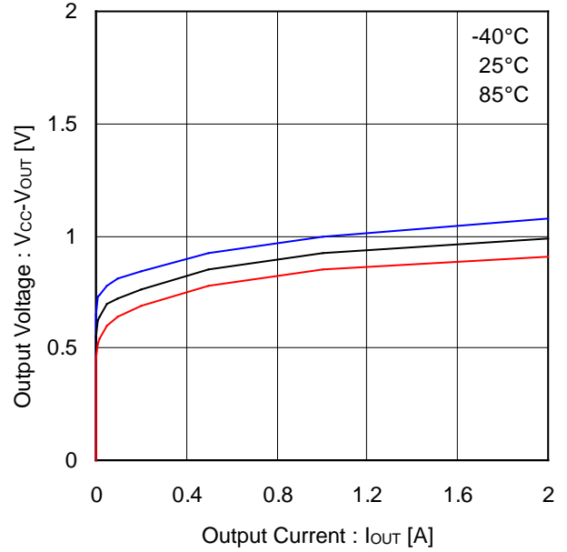
Figure 26. Output Voltage vs Output Current (High Side Body Diode, BD6222)
