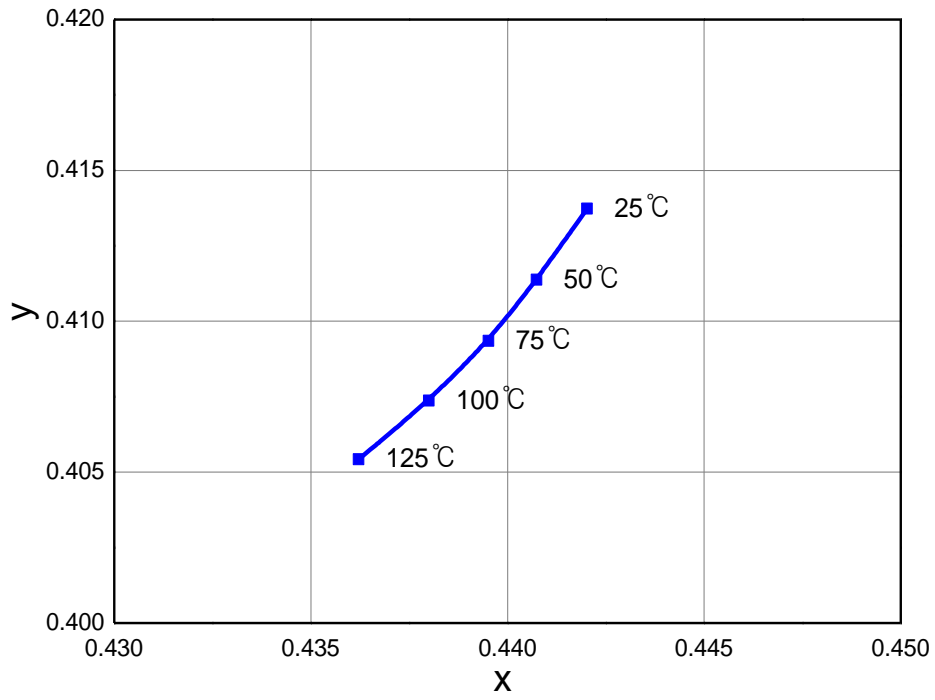
Fig 8. Chromaticity Coordinate vs. Junction Temperature, I_F=20\text{mA}
