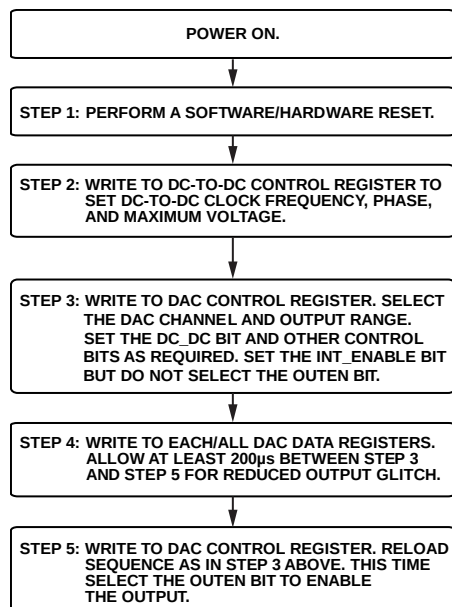
Figure 75. Programming Sequence for Enabling the Output Correctly
