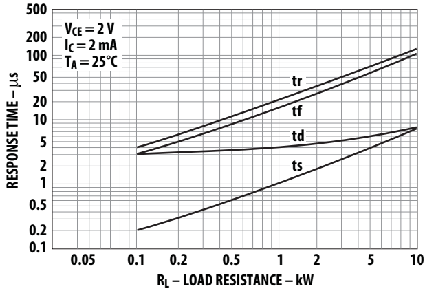
Figure 10. Response time vs. load resistance.
