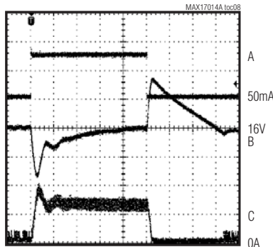
STEP-UP REGULATOR LOAD-TRANSIENT RESPONSE
