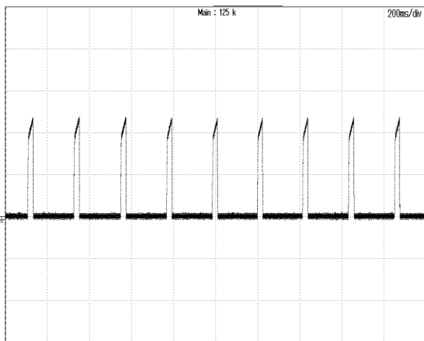
Figure 11: Output short current @Vin=72V CH1:Io, 10A/div, 200mS/div
