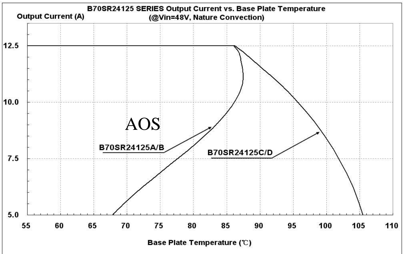
Figure 18: Output Power vs. base plate temperature @Vin=48V
