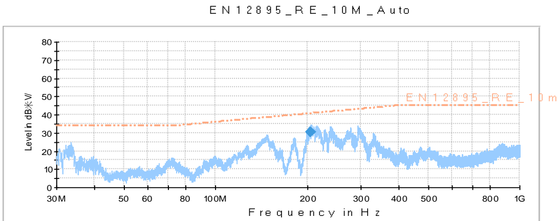
Figure 16: test result(Horizontal)
