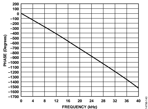
Figure 35. Phase vs. Frequency, 40 kHz Bandwidth, f_s = 96 kHz, Signal Path = DAC_SDATx to ASRC to LOU TLx
