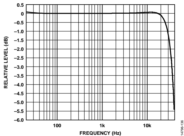
Figure 34. Relative Level vs. Frequency, f_s = 96 kHz, Signal Path = DAC_SDATx to ASRC to LOU TLx
