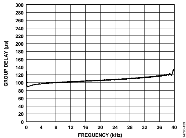
Figure 37. Group Delay vs. Frequency, f_s = 96 kHz, Signal Path = DAC_SDATx to ASRC to LOU TLx
