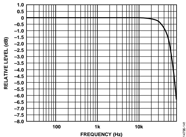
Figure 36. Relative Level vs. Frequency, f_s = 192 kHz, Signal Path = DAC_SDATx to ASRC to LOU TLx
