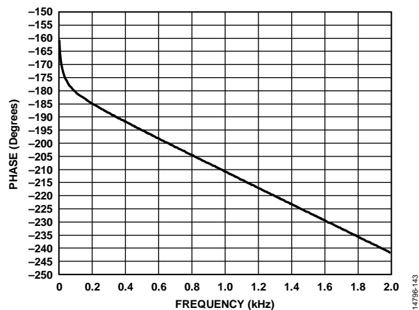
Figure 38. Phase vs. Frequency, 2 kHz Bandwidth, f_s = 96 kHz, Signal Path = DAC_SDATx to ASRC to LOU TLx
