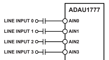
Figure 54. Single-Ended Line Inputs
