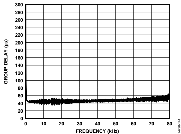
Figure 39. Group Delay vs. Frequency, f_s = 192 kHz, Signal Path = DAC_SDATx to ASRC to LOU TLx
