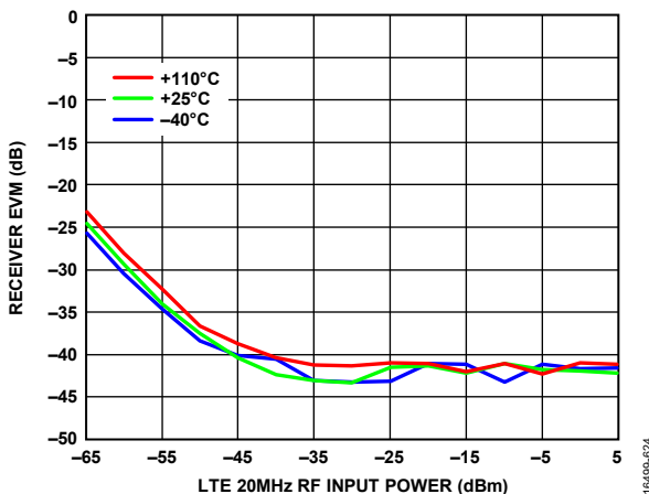
Figure 121. Receiver EVM vs. LTE 20 MHz RF Input Power, LTE 20 MHz RF Signal, LO = 75 MHz, Default AGC Settings
