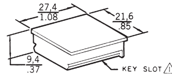
KEY SLOT FACES SIDE OF HOUSING SHOWING CATALOG LISTING (ABOVE LAMP TERMINALS "A" AND "B")
