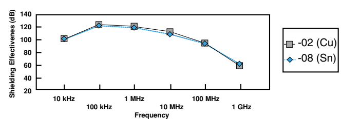
TRANSFER IMPEDANCE PART NO. 0097-0555-XX
