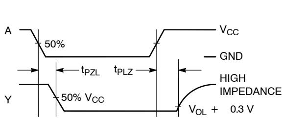
Figure 4. Switching Waveforms
