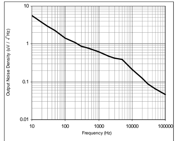
Figure 89. Output Noise Density vs. Frequency
