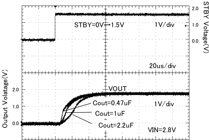
Figure 18. Startup time ( Rout = none )
