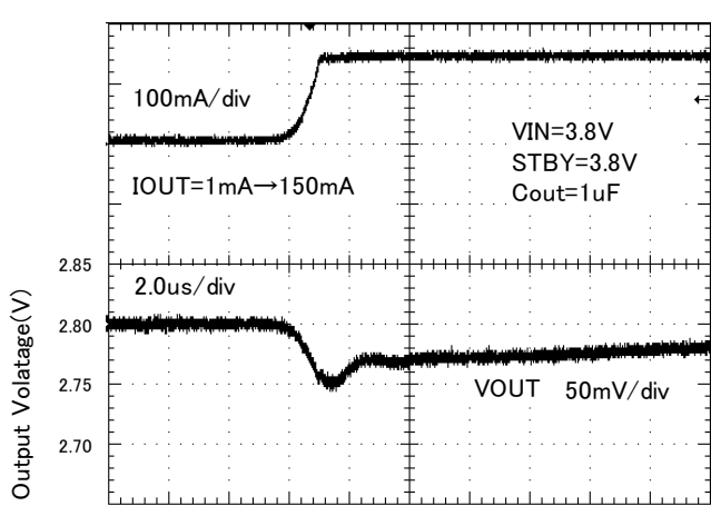
Figure 46. Load response ( I_{out} = 1\text{mA} \rightarrow 150\text{mA} )
