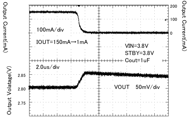
Figure 47. Load response ( I_{out} = 150\text{mA} \rightarrow 1\text{mA} )
