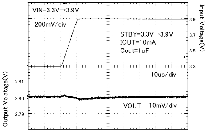
Figure 48. Line response ( V_{in} = 3.3\text{V} \rightarrow 3.9\text{V} )
