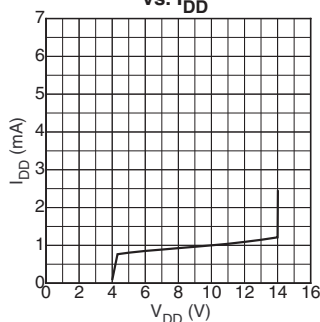
MIC3809 V_{DD} vs. I_{DD}
