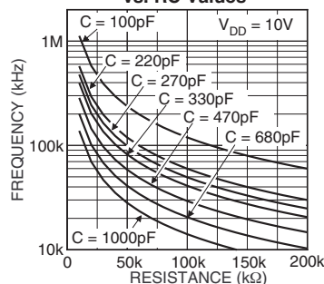
Frequency vs. RC Values
