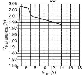
MIC3809 V_{REFERENCE} vs. V_{DD}
