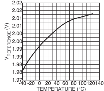
Error Amplifier Reference Voltage vs. Temperature
