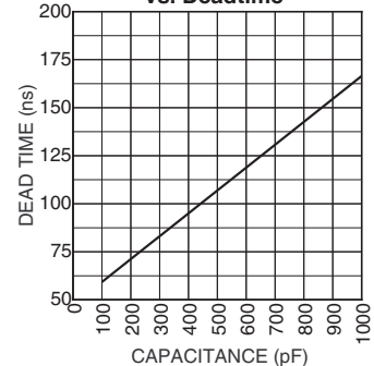
RC Pin Capacitance vs. Deadtime
