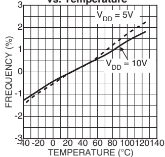
MIC3809 Oscillator Frequency Variation vs. Temperature
