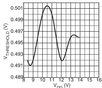
MIC3808 Current Limit Threshold vs. V_{DD}
