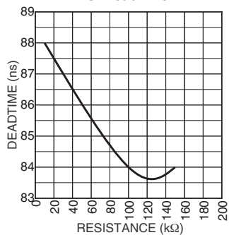
RC Pin Resistance vs. Deadtime
