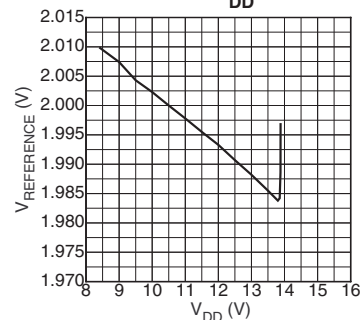
MIC3808 V_{REFERENCE} vs. V_{DD}
