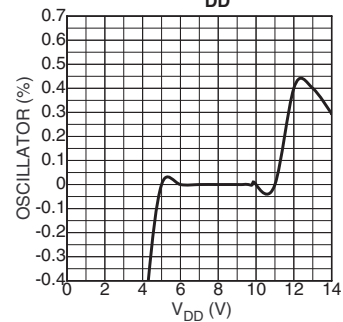
MIC3809 Oscillator Variation vs. V_{DD}
