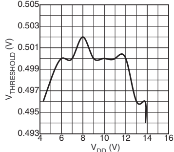
MIC3809 Current Limit Threshold vs. V_{DD}
