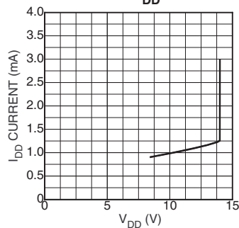
MIC3808 V_{DD} vs. I_{DD}
