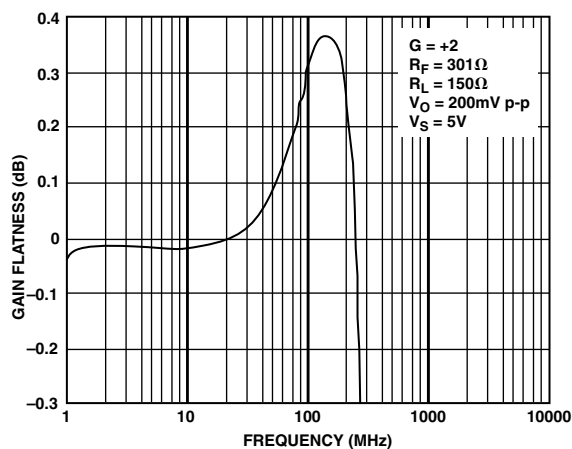
TPC 5. Gain Flatness; G = +2 ; V_S = 5\text{V}
