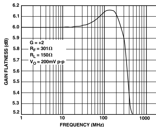
TPC 4. Gain Flatness; G = +2
