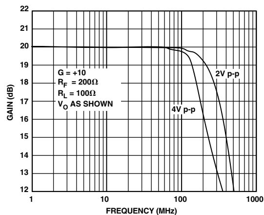
TPC 6. Large Signal Frequency Response; G = +10
