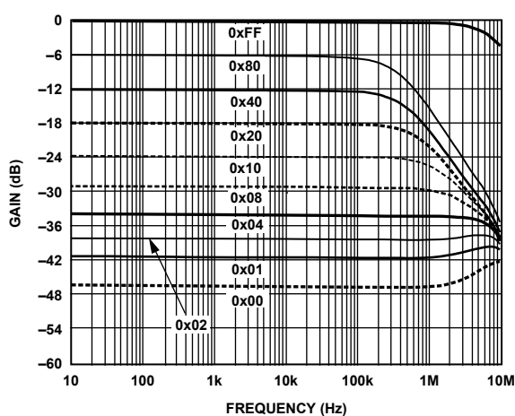
Figure 14. Gain vs. Frequency vs. Code, R_{AB} = 10k\Omega , T_A = 25^\circ C
