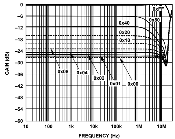
Figure 13. Gain vs. Frequency vs. Code, R_{AB} = 1k\Omega , T_A = 25^\circ C
