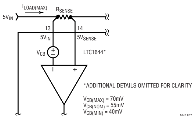
Figure 7. Circuit Breaker Equivalent Circuit for Calculating R_{\text{SENSE}}
